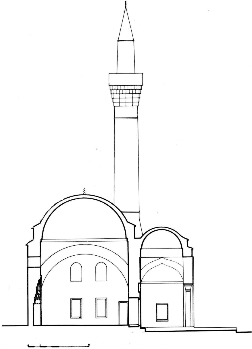
Tire, Kazanoğlu Camii kesit. Tire, Kazanoğlu Mosque section.
